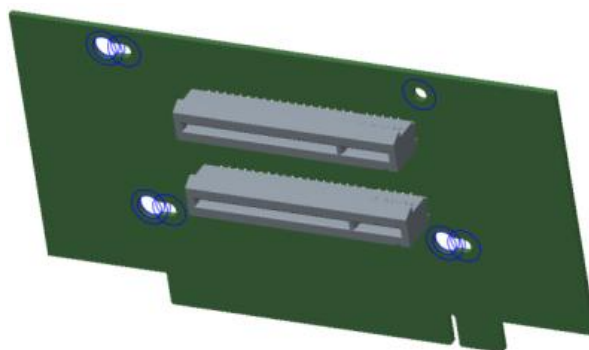
Figure 86. Low profile riser card (iPC – A2UX8X4RISER)
