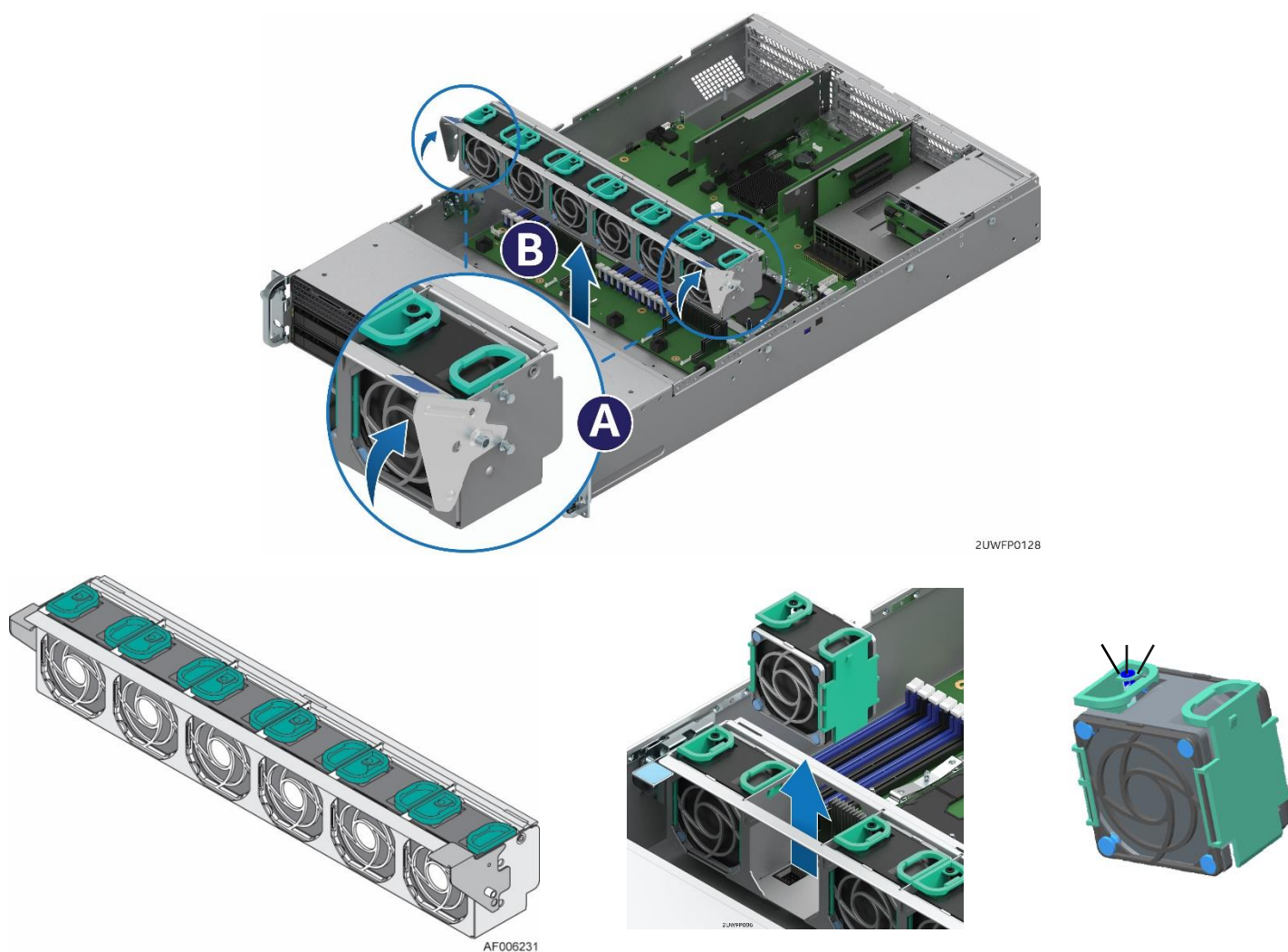
Figure 34. System fan assembly
