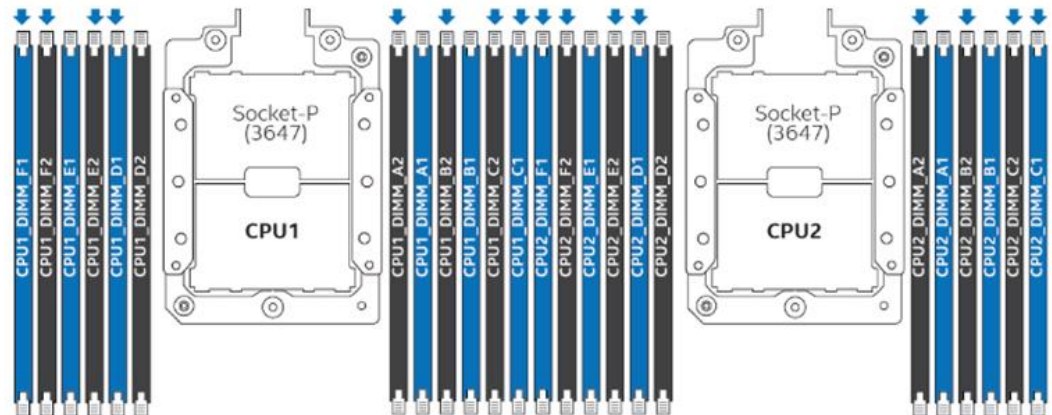
Figure 31. System DIMM/DIMM blanks for 24x2.5 and 12x3.5 drive configurations
