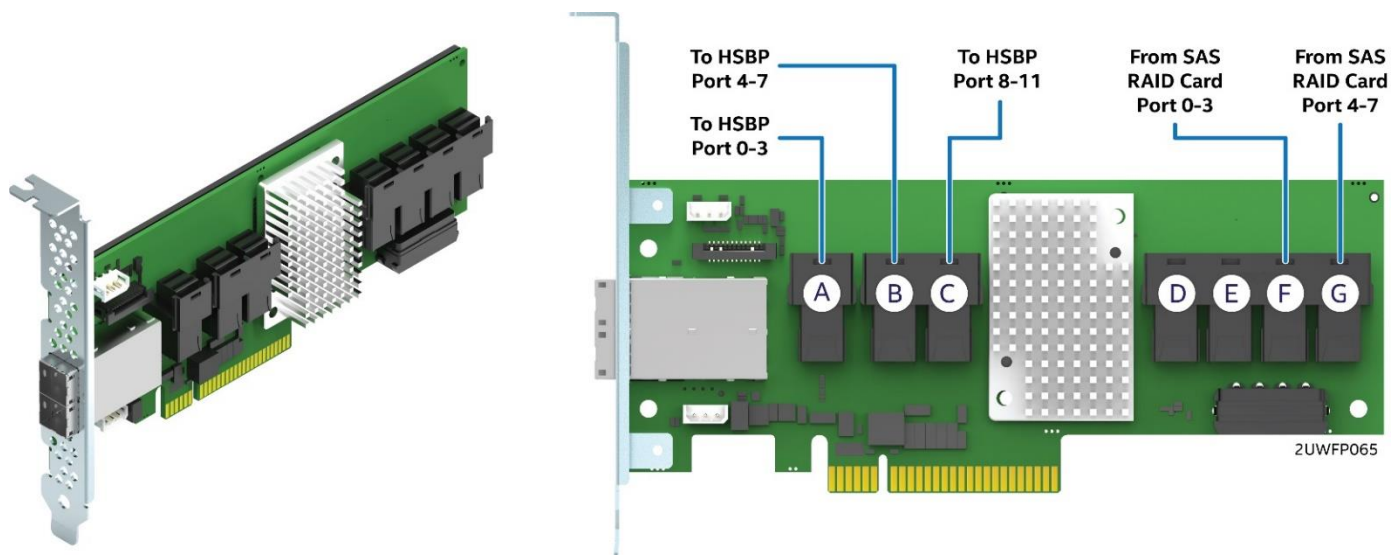
Figure 76. Intel® RAID Expander RES3FV288 connector identification
