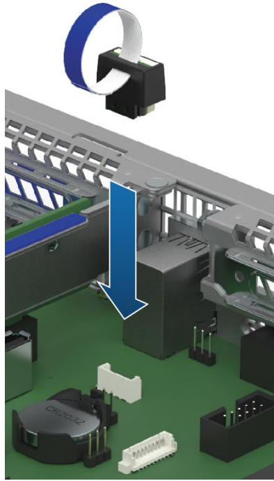
Figure 63. ESRT2 SATA RAID-5 upgrade key
