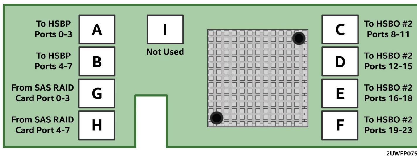
Figure 77. 12 GB internal 36-Port Intel® RAID Expander Card RES3TV360 connector identification
