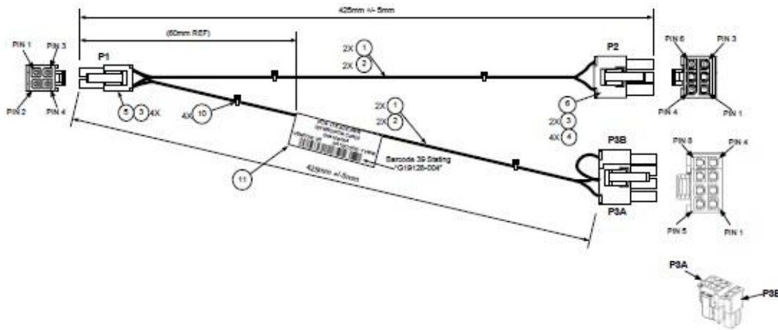
Figure 36. Auxiliary 12 V power cable (iPC – AXXGPGPUCABLE)
