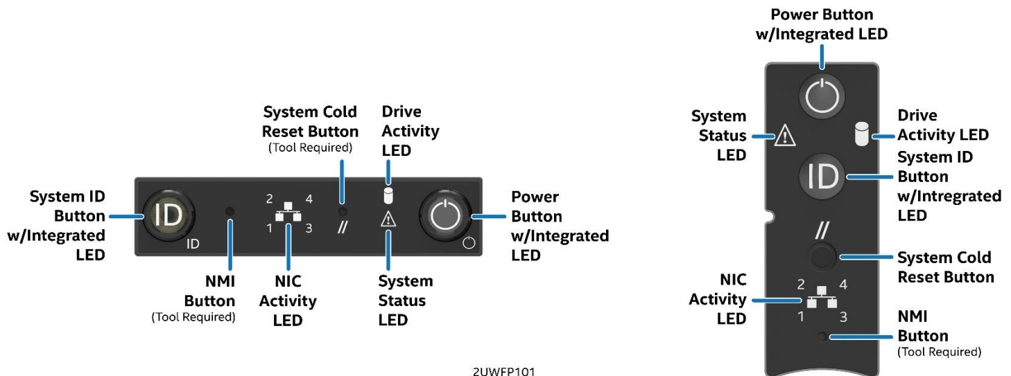
Figure 79. Front control panel features
