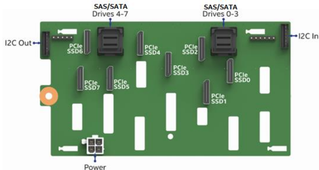
Figure 51. 8 x 2.5" SAS/SATA/NVMe* hot swap backplane, back side
