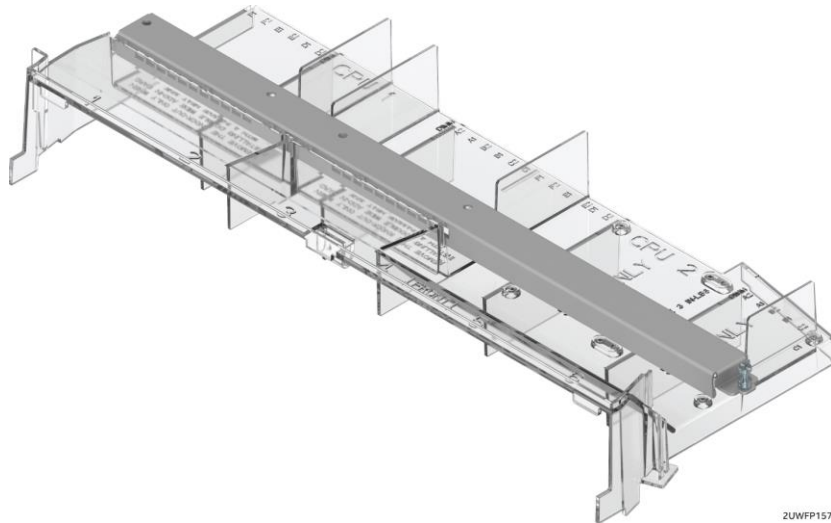
Figure 39. Shipping bracket placement
