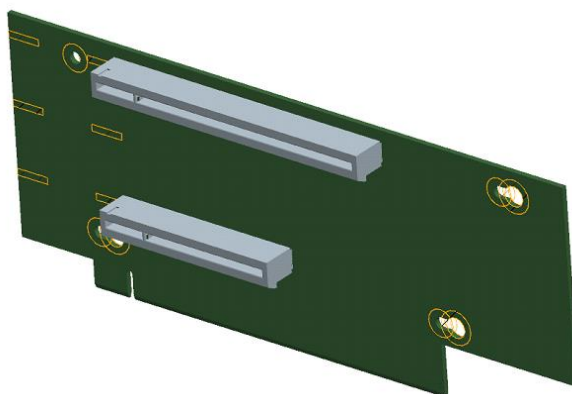
Figure 85. Two-slot PCIe riser card (iPC – A2UL16RISER2)
