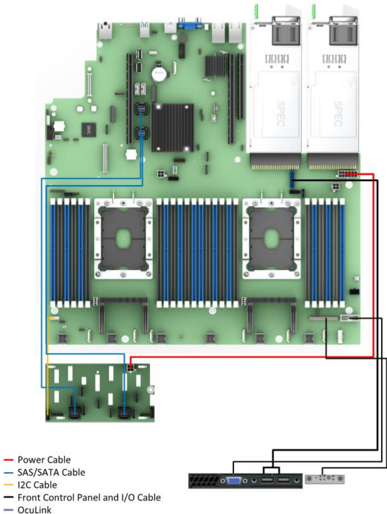
Figure 92. R2208WFxxx system cable routing diagram
