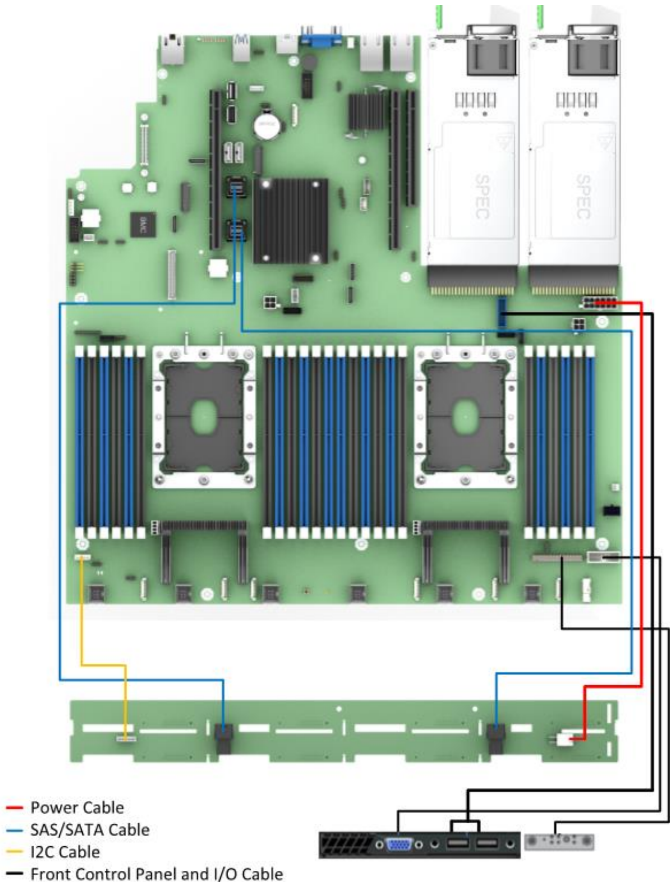
Figure 91. R2308WFxxx system cable routing diagram
