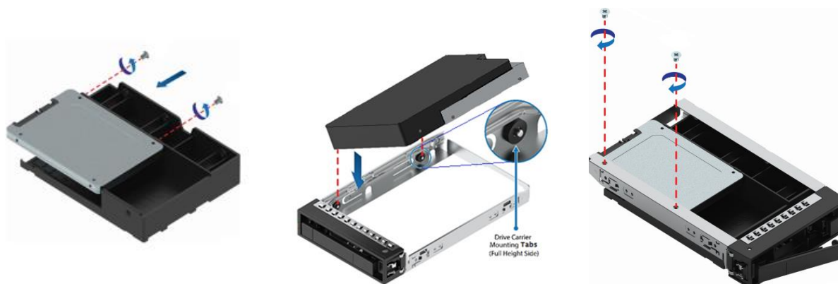
Figure 45. 2.5" SSD mounted to 3.5" drive carrier
