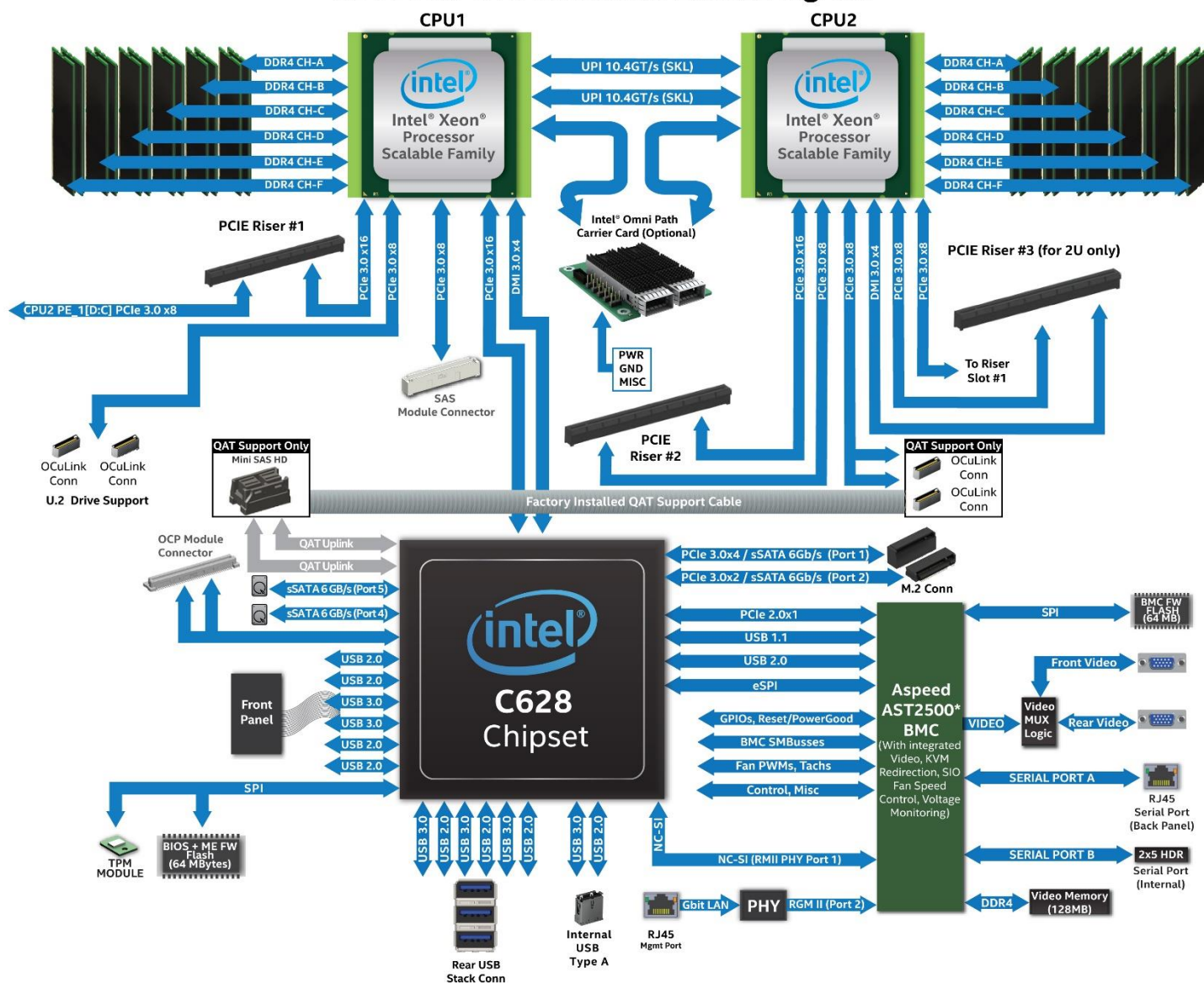
Figure 4. S2600WFQ Server Board Architecture
