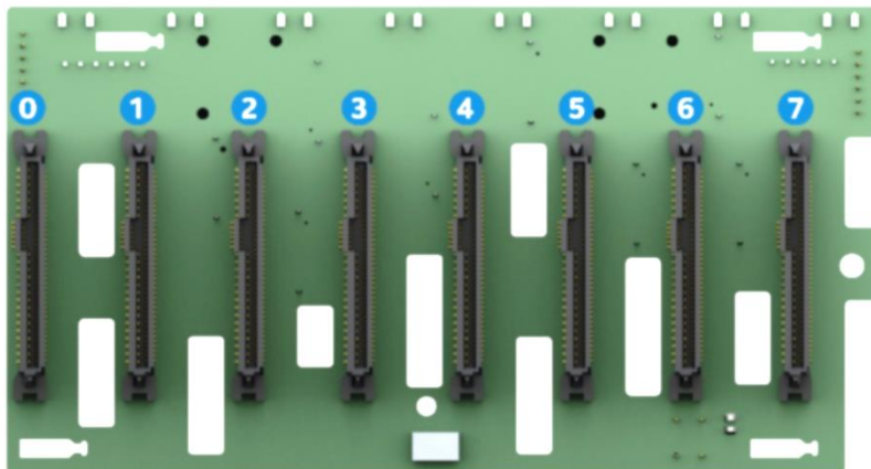
Figure 50. 8 x 2.5" SAS/SATA/NVMe* hot swap backplane, front side
