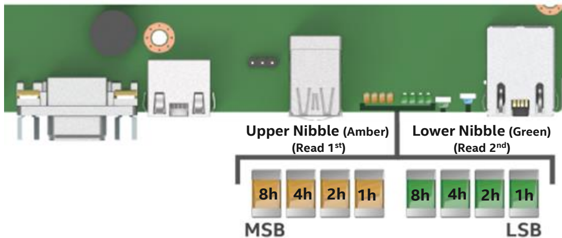
Figure 90. On-board POST Diagnostic LEDs
