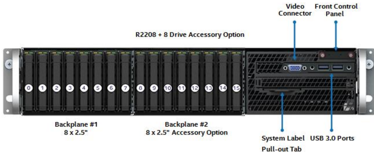
Figure 40. 2.5" front mount drive bay, 8 drive (R2208WFxxx) and 16 drive configuration option
