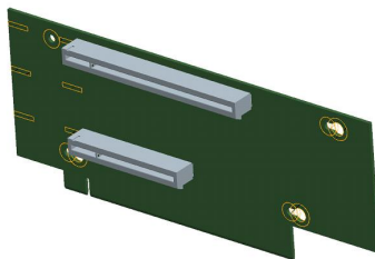
Figure 35. 2-slot PCIe* riser card
