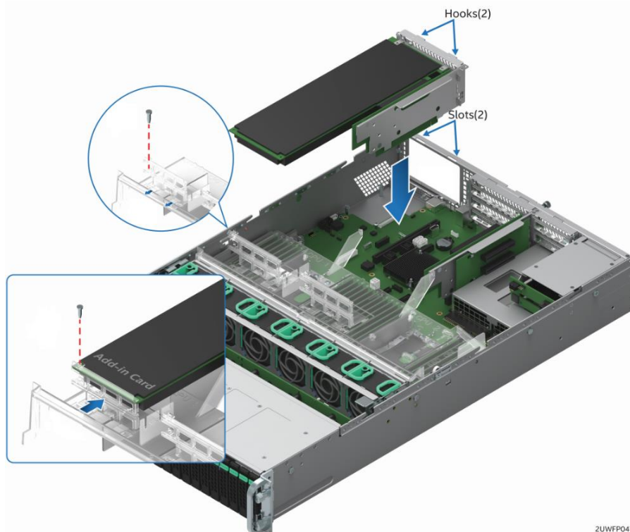
Figure 83. Full height/full length add-in card support
