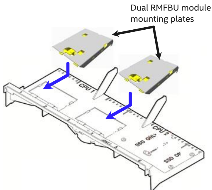
Figure 74. Dual RMFBU mounting bracket installation
