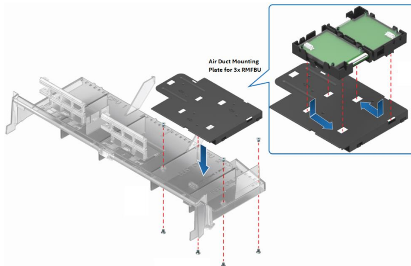
Figure 73. Triple RMFBU (default) mounting bracket installation
