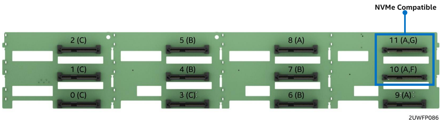
Figure 56. 12 x 3.5" hot swap backplane, front side
