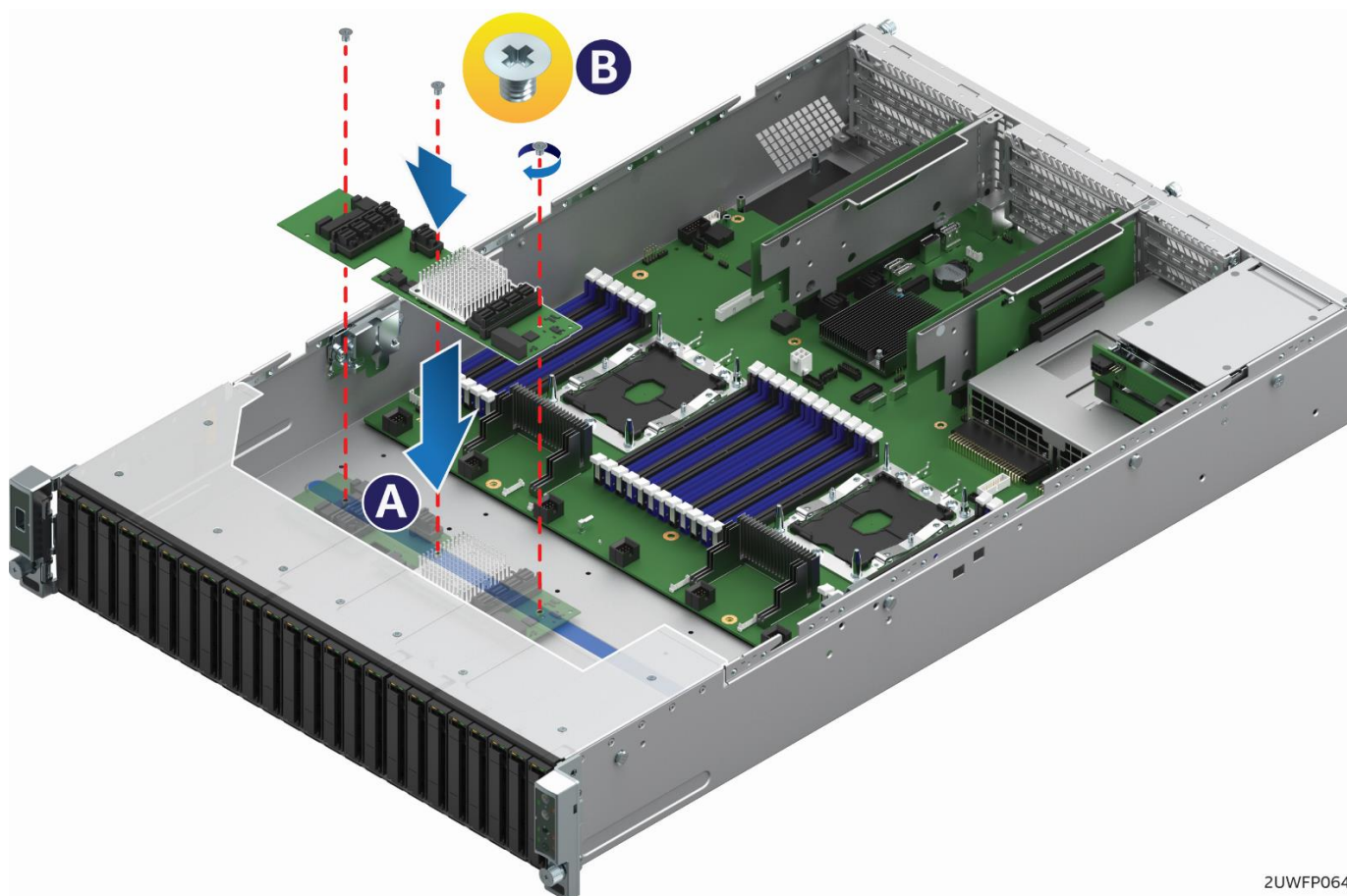
Figure 75. SAS expander card installation
