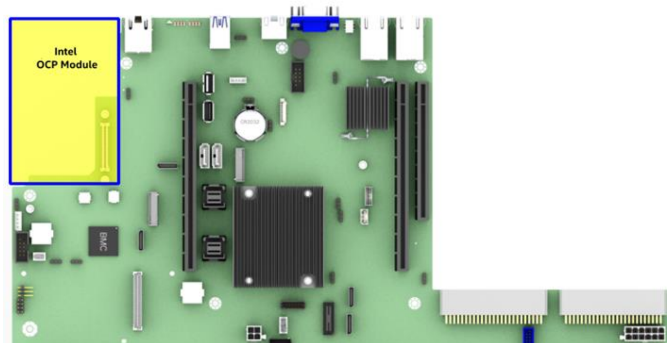
Figure 87. OCP module placement
