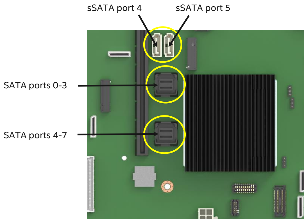
Figure 61. Onboard storage support features
