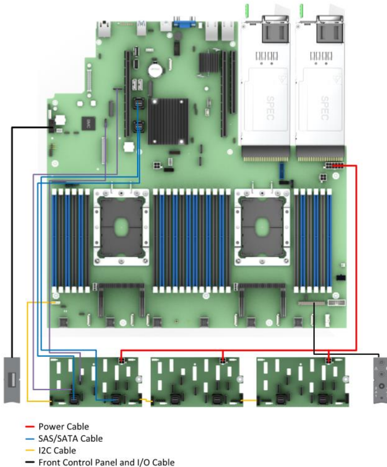
Figure 95. R2224WFxxx system cable routing diagram
