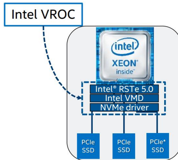
Figure 69. Intel® VROC basic architecture overview
