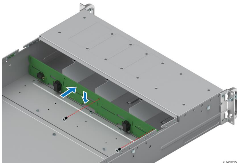
Figure 48. 3.5" backplane placement
