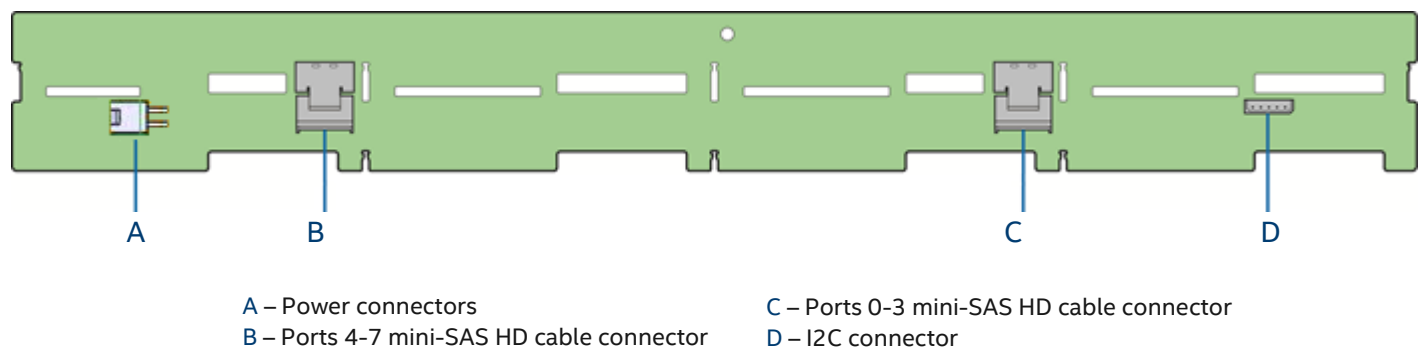
Figure 55. 8 x 3.5" HSBP Connector Identification
