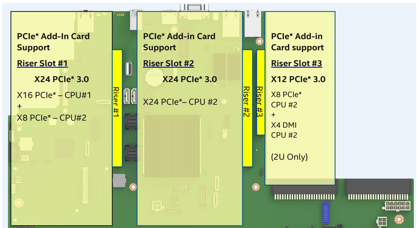
Figure 80. PCIe* add-in card support
