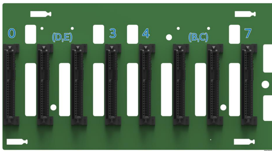
Figure 53. 8 x 2.5" dual port SAS backplane, front side
