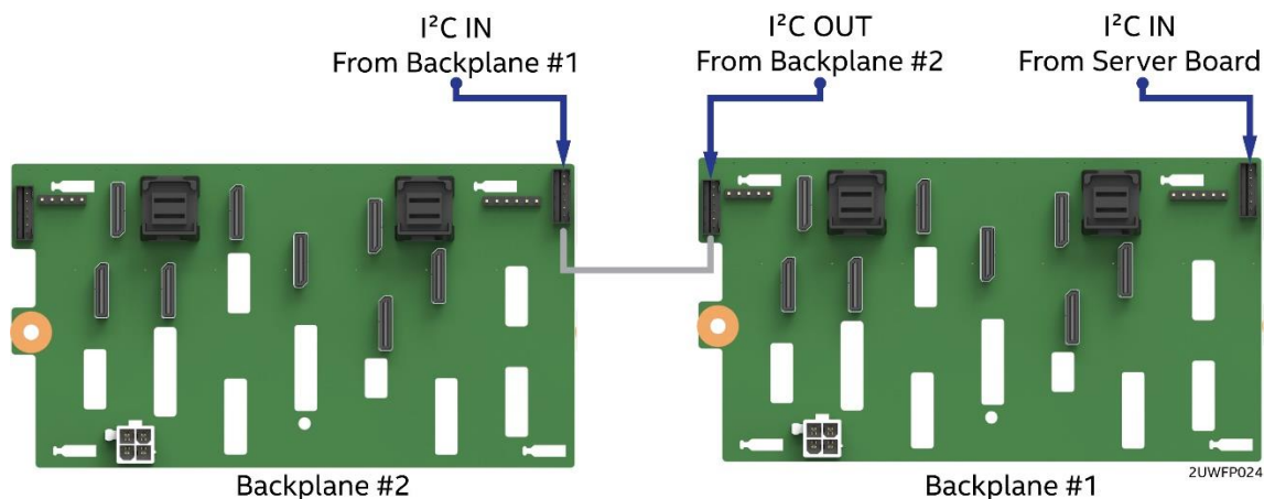
Figure 52. 8 x 2.5" dual port SAS backplane, back side
