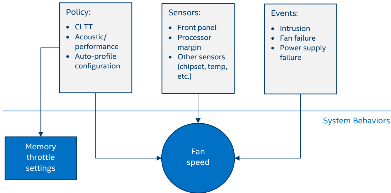
Figure 32. High-level fan speed control model
