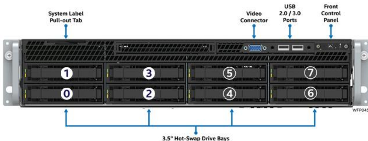
Figure 42. 3.5" drive bay, 8 drive configuration
