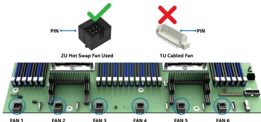
Figure 33. Server board 2U system fan connector locations
