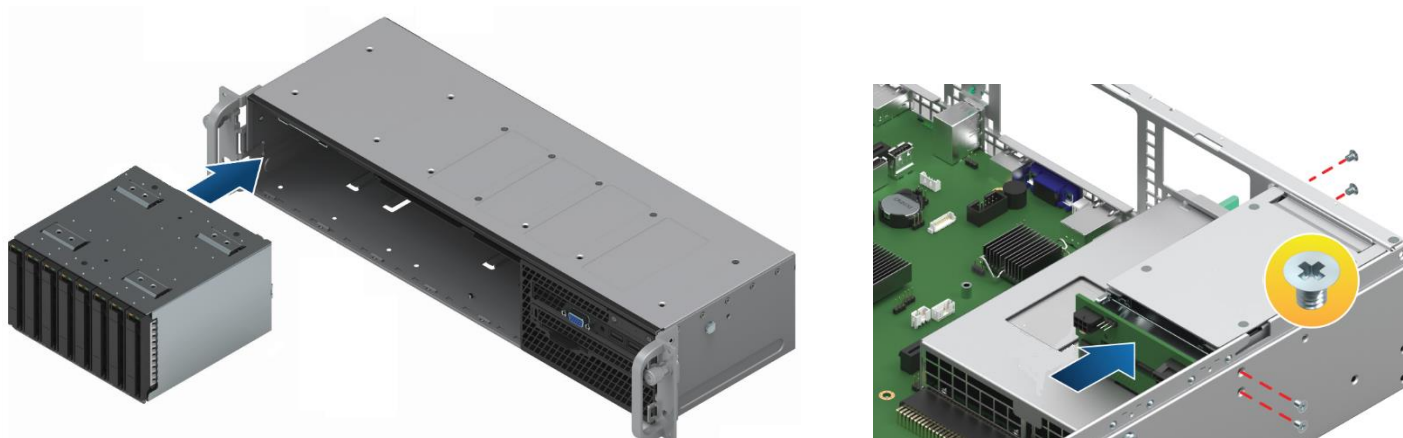
Figure 49. 2.5" drive bay module placement options
