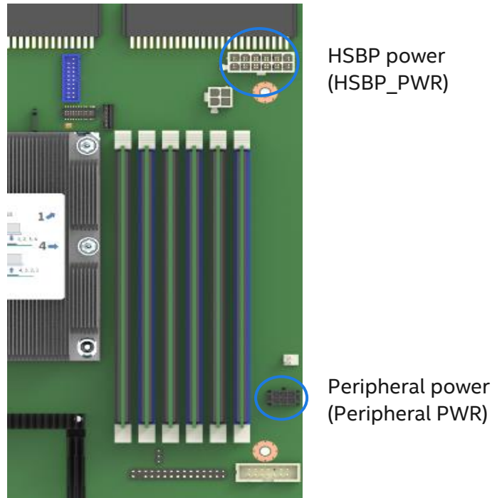
Figure 47. Server board peripheral power connectors
