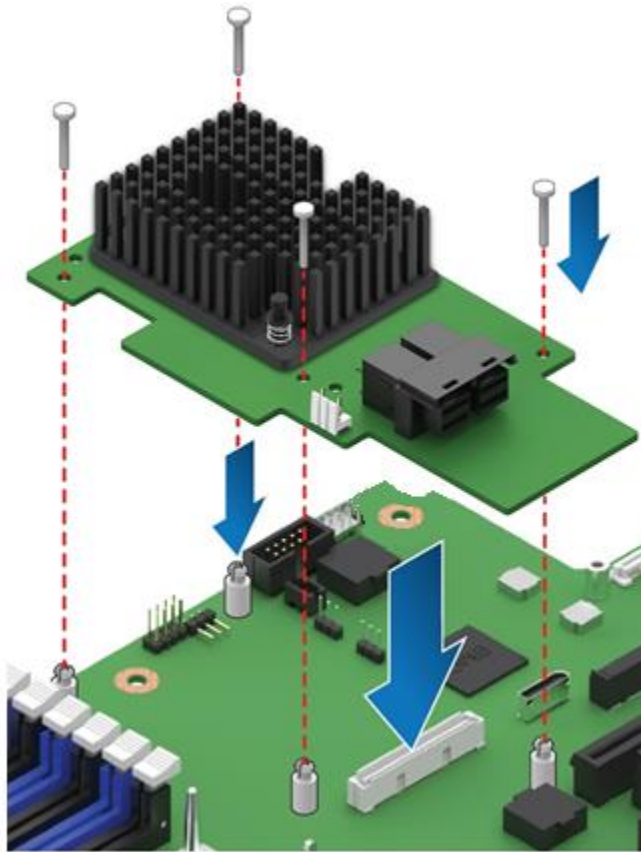
Figure 72. Intel® Integrated RAID Module
